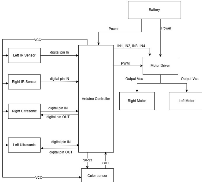
Fig. 2. Block diagram of the robot system architecture.
